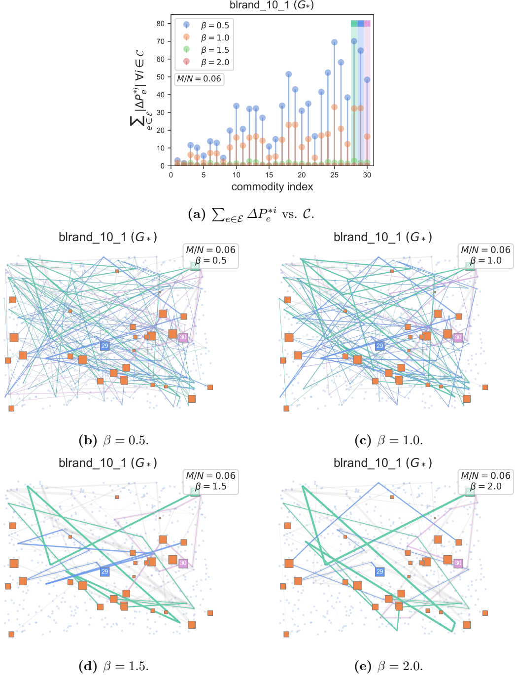
Figure 1.5: Panels (a): \sum_{e \in \mathcal{E}} |\Delta P_e^{*i}| vs. \mathcal{C} . Panel (b-e): Qualitative explanation of non-trivial interaction among commodities. \ell_e = 1 + \varepsilon 10^{-3} , \varepsilon \sim U(0, 1) , the position of each node is sampled at random in the square [0, 1] \times [0, 1] for visualization purpose. MCOT, mesh: bland_10_1, N = 500 , M = 30 , E = 1020 , \beta \in \{0.5, 1.0, 1.5, 2.0\} . Results computed on one single instance, keeping \{g^i\}^i and \{f^i\}^i fixed for every \beta . Similar plots for M = 40, 50 are in figs. A.1i and A.1j in appendix A.
