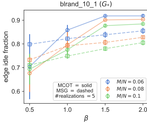
Figure 1.8: idle edge fraction vs. \beta . Mesh: blrand_10_1 , N = 500 , M = 30, 40, 50 , E = 1020 . Results averaged over 5 realizations.
