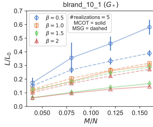
Figure 1.10: L/L_0 vs. M/N . Mesh: blrand_10_1 , N = 500 , \beta \in \{0.5, 1.0, 1.5, 2.0\} , E = 1020 . Results averaged over 5 realizations.
