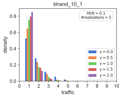
Figure 1.6: Histograms showing the traffic distribution on \mathcal{E} for different values of \gamma . MSG, mesh: blrand_10_1 , N = 500 , M = 50 , E = 1020 , \gamma \in \{0.0, 0.5, 1.0, 1.5, 2.0\} . Results averaged over 5 realizations. Similar plots for M = 30, 40 are in figs. A.1k and A.1l in appendix A.
