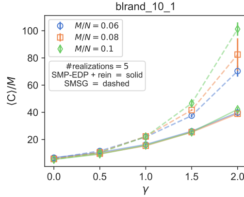
Figure 2.11: \langle C \rangle vs. \gamma . Mesh: blrand_10_1 , N = 500 , M = 30, 40, 50 , E = 1020 . Results averaged over 5 realizations.
