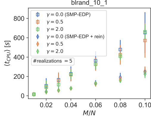
Figure 2.4: \langle t_{CPU} \rangle vs. M/N . SMP-EDP, mesh: brand_10_1 , N = 500 , \gamma \in \{0.0, 0.5, 2.0\} , E = 1020 . Results averaged over 5 realizations.
