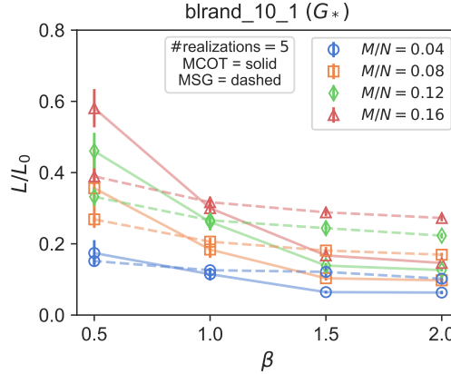
Figure 1.9: L/L_0 vs. \beta . Mesh: blrand_10_1 , N = 500 , M = 30, 40, 50 , E = 1020 . Results averaged over 5 realizations.
