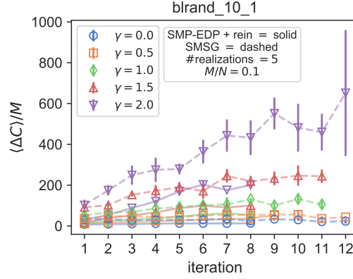
Figure 2.10: \langle \Delta C / M_{acc} \rangle vs. iteration. Mesh: blrand_10_1 , \gamma \in \{0.0, 0.5, 1.0, 1.5, 2.0\} , E = 1020 . Results averaged over 5 realizations. Similar plots are in figs. B.1g and B.1h in appendix B.
