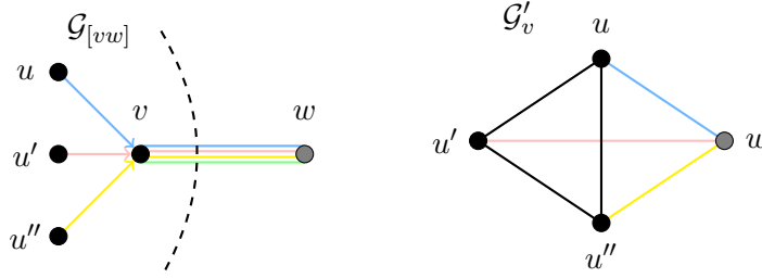
Figure 2.2: Building the auxiliary complete graph \mathcal{G}'_v .
