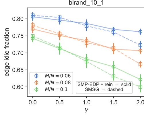
Figure 2.12: idle edge fraction vs. \gamma . Mesh: bland_10_1, N = 500 , M = 30, 40, 50 , E = 1020 . Results averaged over 5 realizations.
